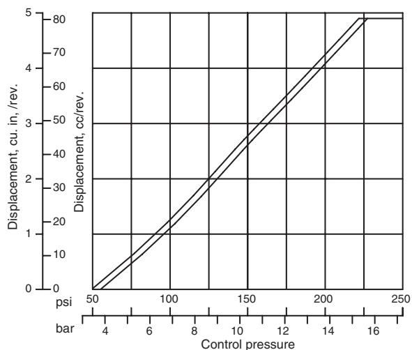
HYDRAULIC STROKER
